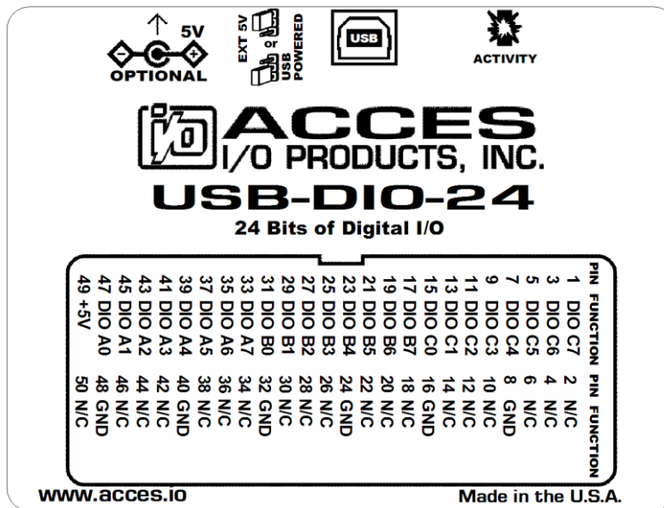
Figure 1-3: USB-DIO-24 Enclosure Label
