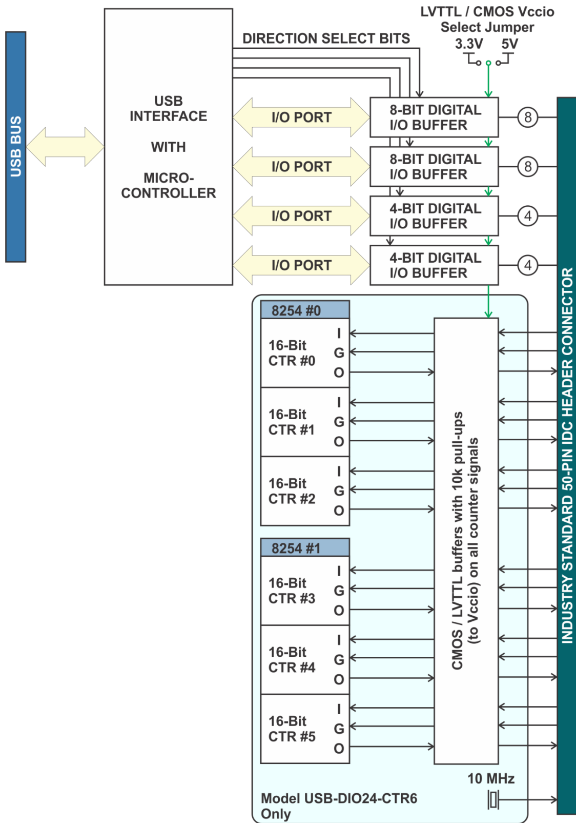
Figure 1-1: Block Diagram
