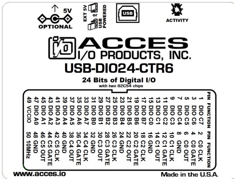
Figure 1-2: USB-DIO24-CTR6 Enclosure Label
